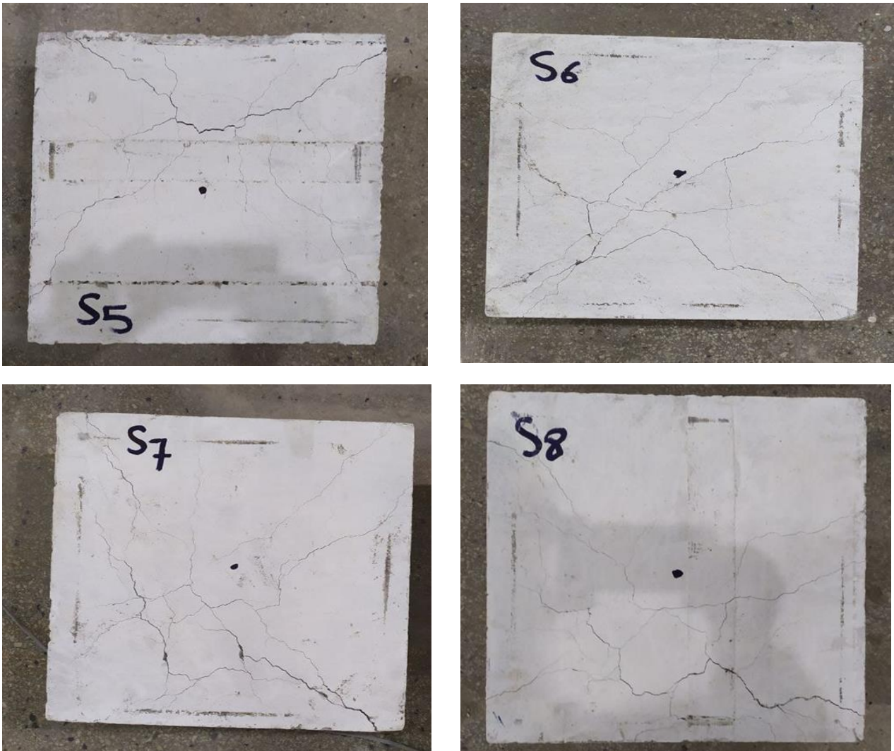
Figure 9. The tested slabs' crack pattern and mode of failure group 2
