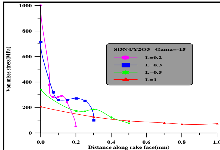
Fig. (8): distribution of Von Mises stress along rake face (primary rake angle = -15^{\circ} and material tool \text{Si}_3\text{N}_4/\text{Y}_2\text{O}_3 ).
