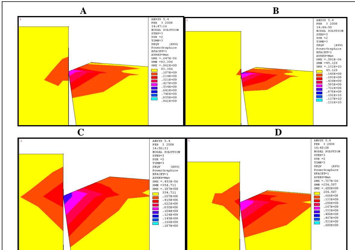
Fig. (17): effect of rake angle ( -25^\circ ) and different land width on Von Mises stresses for Al_2O_3/TiC tool material.
