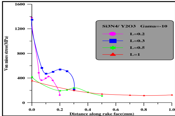
Fig. (5): distribution of Von Mises stress along rake face ( \gamma = -10^\circ and material tool Si3N4/Y 2 O 3 ).
