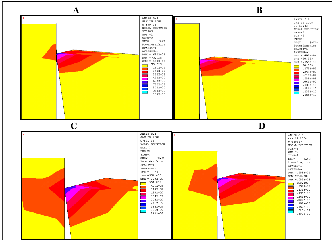
Fig. (13): effect of rake angle (-15) and different land width on Von Mises stresses for AL_2O_3/ZrO_2 tool material.
