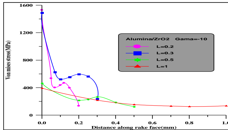
Fig. (3): distribution of Von Mises stress along rake face ( \gamma = -10^\circ and material tool Al_2O_3/ZrO_2 ).
