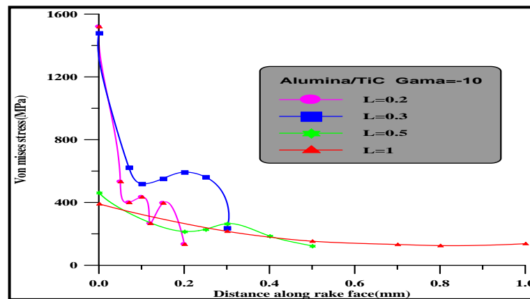
Fig. (4): distribution of Von Mises stress along rake face (primary rake angle = -10^\circ and material tool Al_2O_3/TiC ).
