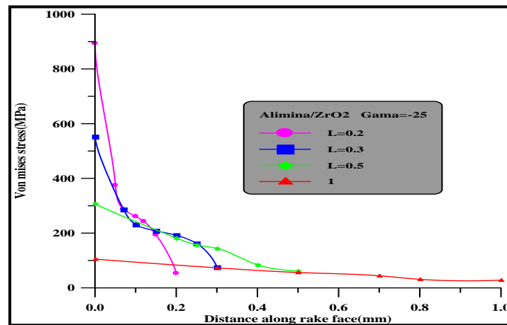
Fig.(9): distribution of Von Mises stress along rake face ( \gamma = -25^{\circ} and material tool \text{Al}_2\text{O}_3/\text{ZrO}_2 ).
