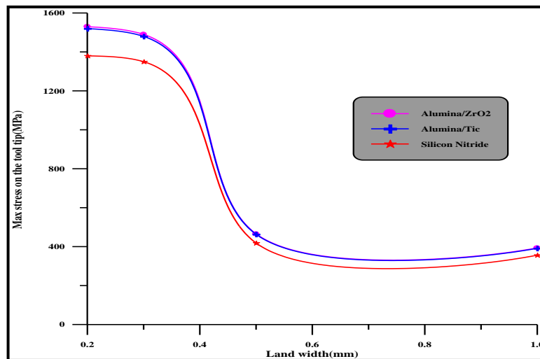
Fig. (21): the relation of maximum stress on the cutting tool and land width for different materials of ceramic cutting tools.
