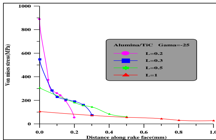
Fig.(10): distribution of Von Mises stress along rake face (primary rake angle = -25^{\circ} and material tool \text{Al}_2\text{O}_3/\text{TiC} ).
