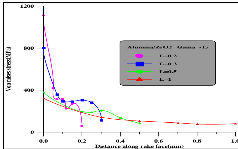
Fig. (6): distribution of Von Mises stress along rake face (primary rake angle = -15^\circ and material tool AL 2 O 3 /ZrO 2 ).
