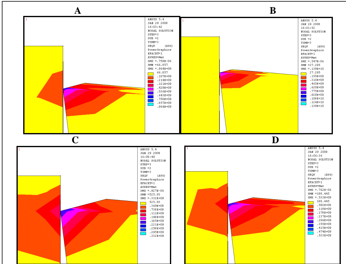
Fig. (19): effect of rake angle ( -15^\circ ) and different land width on Von Mises stresses for Si3N4/Y2O3 tool material.
