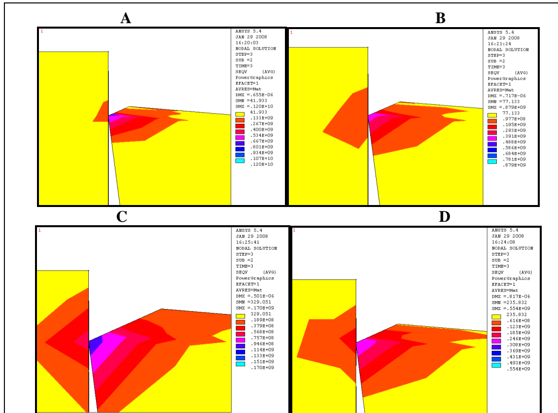
Fig. (20): effect of rake angle ( -25^\circ ) and different land width on Von Mises stresses for Si3N4/Y2O3 tool material.
