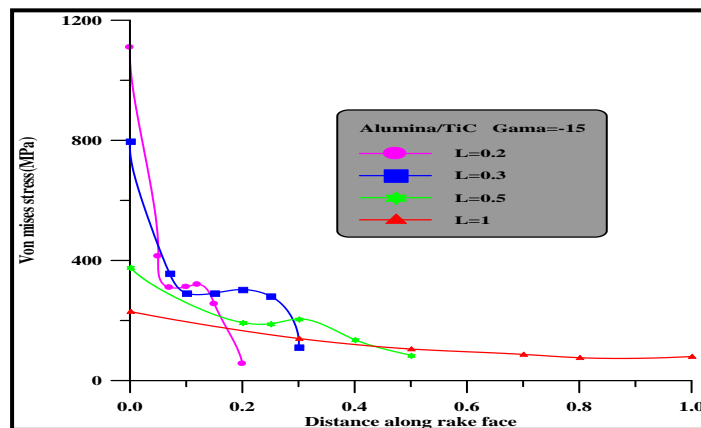
Fig. (7): distribution of Von Mises stress along rake face ( \gamma = -15^\circ and material tool AL 2 O 3 /TiC).
