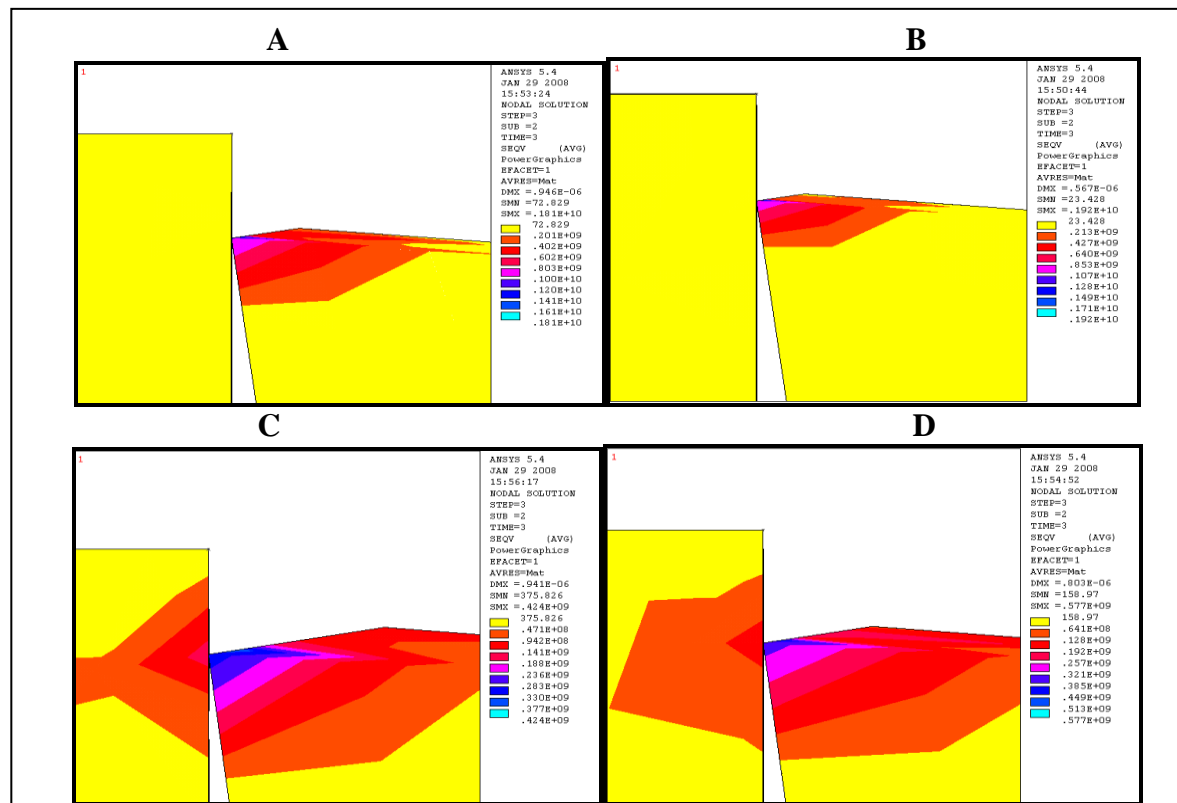
Fig. (18): effect of rake angle ( -10^\circ ) and different land width on Von Mises stresses for Si_3N_4/Y_2O_3 tool material.
