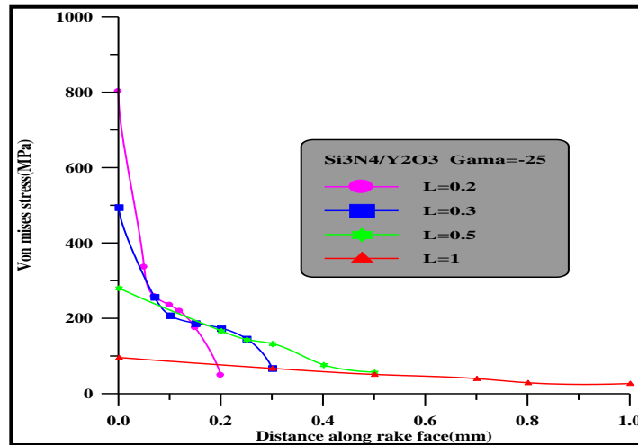
Fig. (11): distribution of Von Mises stress along rake face (primary rake angle = -25^{\circ} and material tool \text{Si}_3\text{N}_4/\text{Y}_2\text{O}_3 ).
