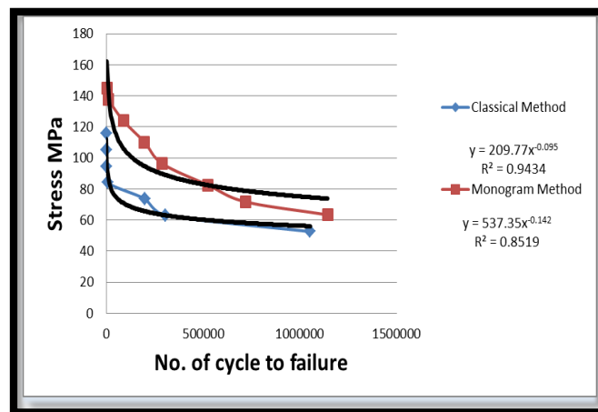
Figure 9. S-N curve
